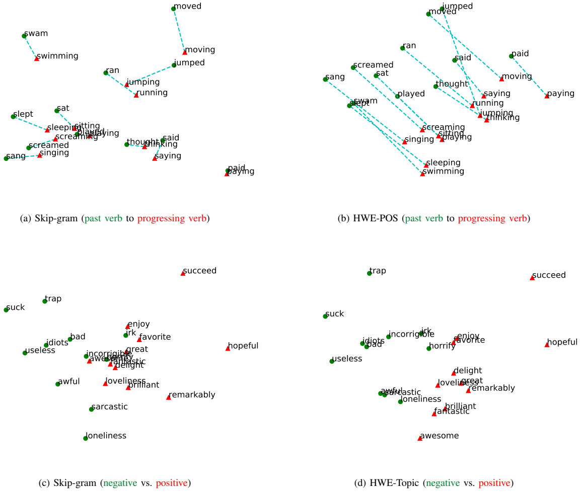
Fig. 3: (Top) 2-dimensional PCA projection for word pairs holding the past verb to progressing verb relations. (Bottom) 2-dimensional PCA projection for the negative and positive affective terms .
